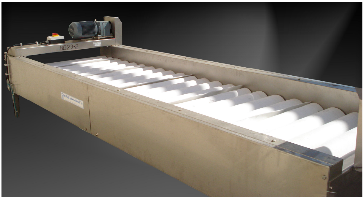
Roller dryer RD23-R2
